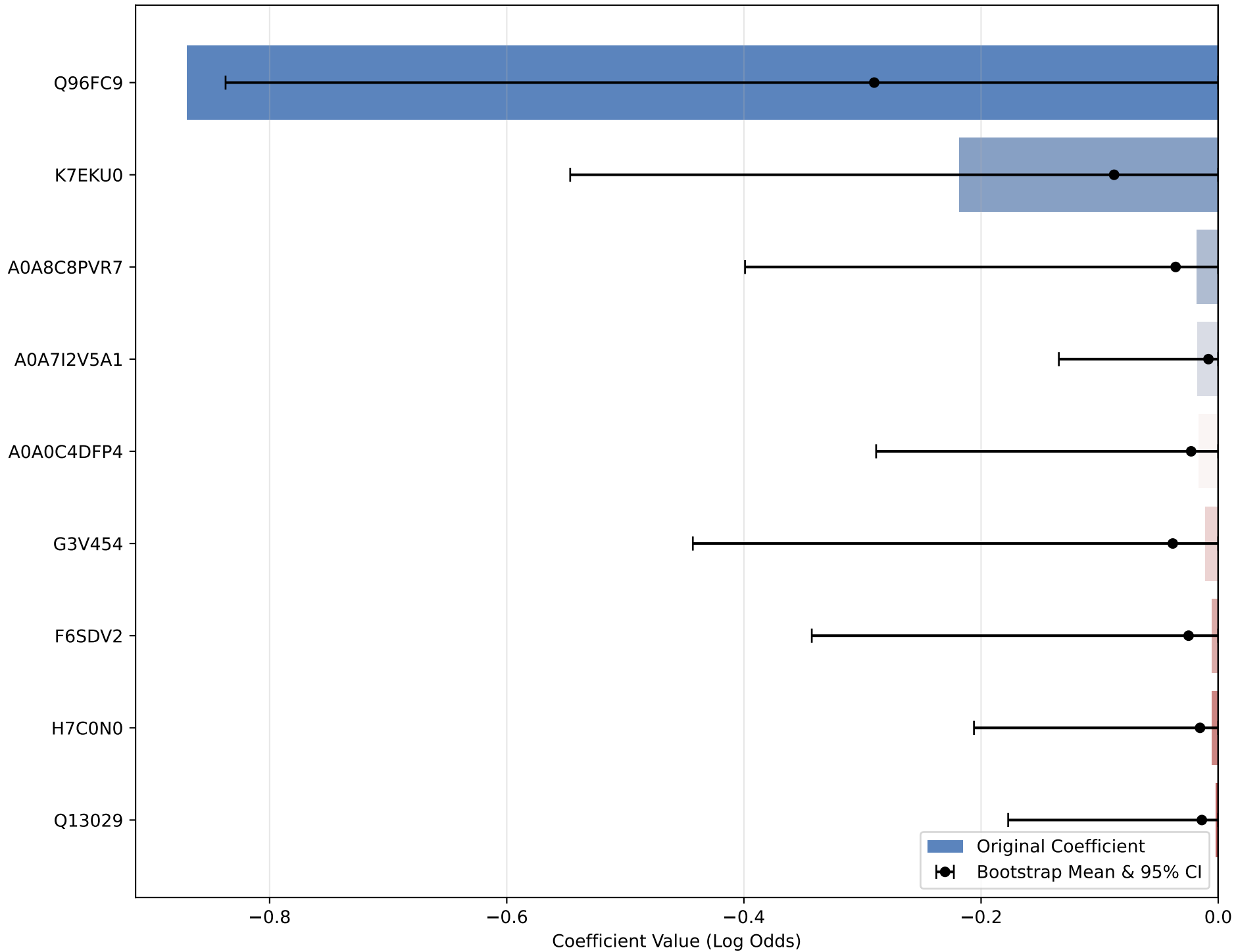
Top 9 Features (Bars = Original, Points/Lines = Bootstrap 95% CI)
